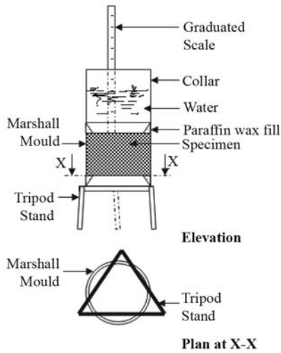
Fig. 4. Typical permeability test setup
