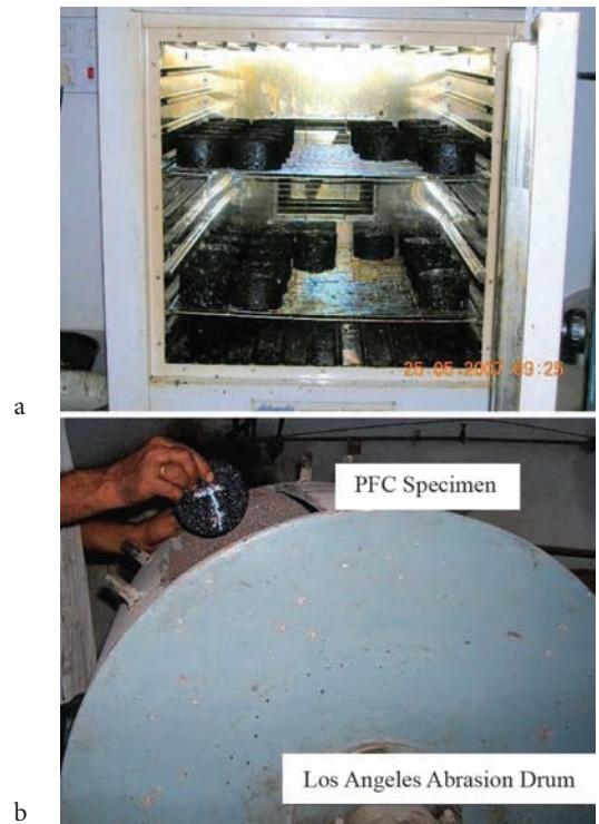
Fig. 6. Specimens subjected to aging in a hot air oven (a) and abrasion test (b)
