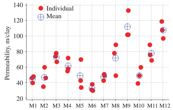
Fig. 5. Results of permeability tests on all 12 mixes
