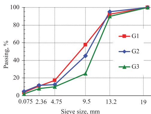
Fig. 1. Gradations investigated for PFC mixes
