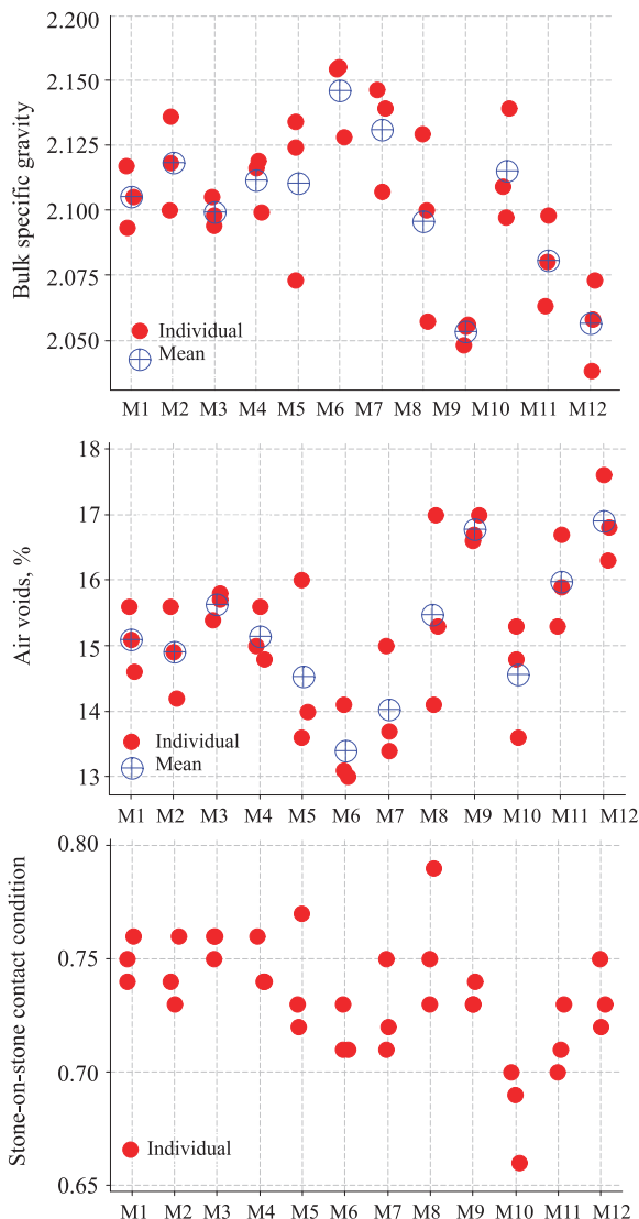
Fig. 3. Individual plot for volumetric properties of all 12 mixes
