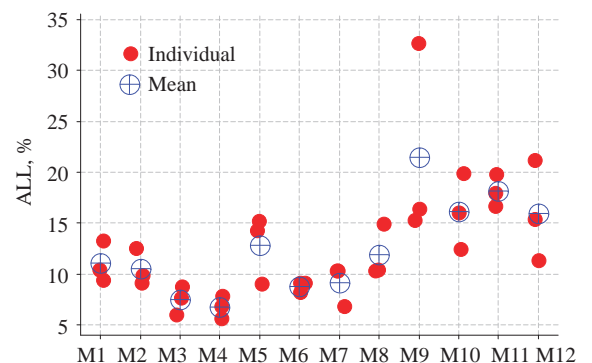
Fig. 7. Results of ALL tests on all 12 mixes
