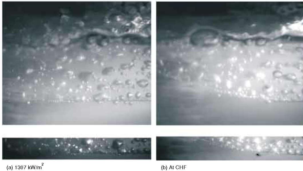
Figure 10. (a) Massive vapour bubbles appear on the surface of the test wire exposed to 1307 kW/m 2 heat input continuously and leave the surface. Bubble density is also higher; (b) Bubbles grow in size when the heat flux was increased to CHF value, of 1408 kW/m 2
